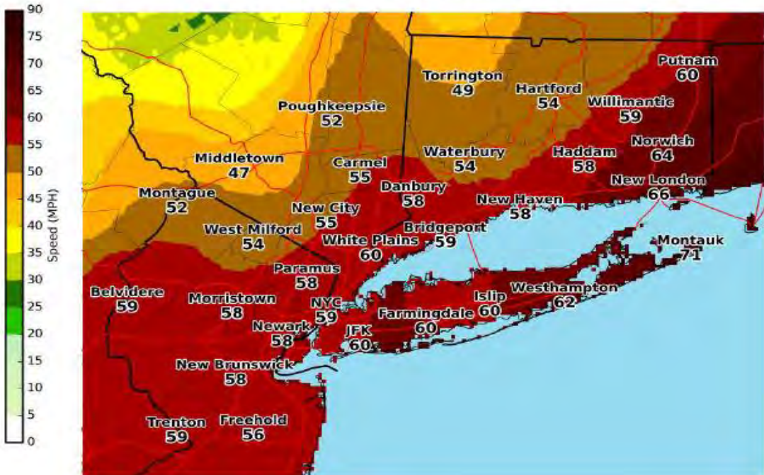
Wind Gusts Valid: Friday, March 02, 2018 at 04 PM EST
